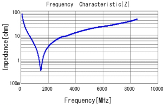
■ GRM1882C1H220JA01 |Z| DCOV, 20degC
