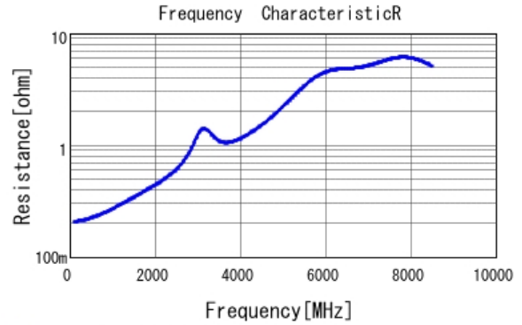
■ GRM1882C1H220JA01 R DCOV, 20degC
