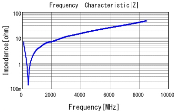
■ GRM1882C1H221JA01 |Z| DCOV, 20degC
