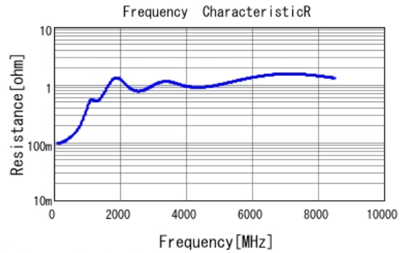
■ GRM1882C1H221JA01 R DCOV, 20degC
