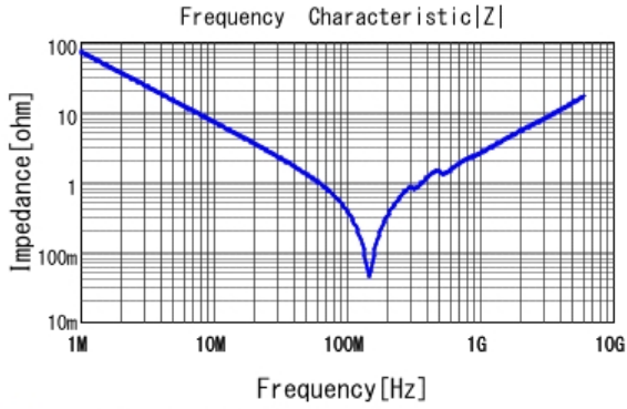
■ GRM1882C1H222JA01 |Z| DCOV, 20degC
