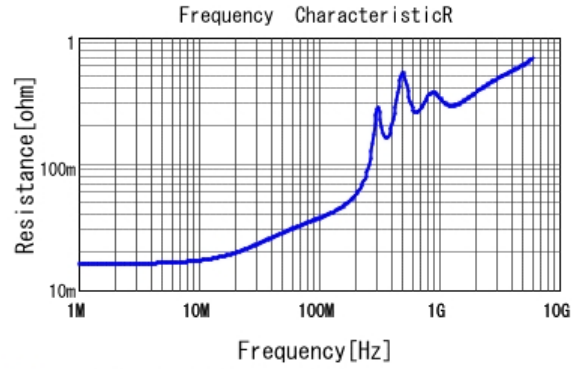
■ GRM1882C1H222JA01 R DCOV, 20degC
