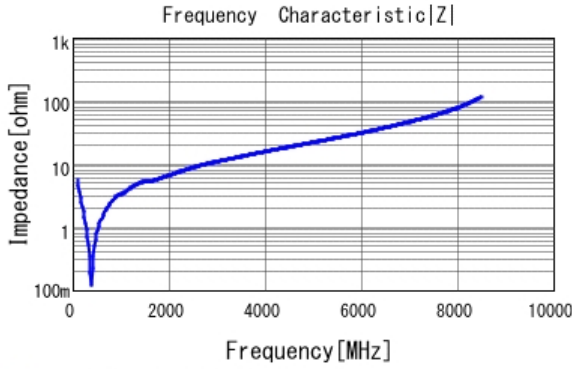
■ GRM1882C1H271JA01 |Z| DCOV, 20degC
