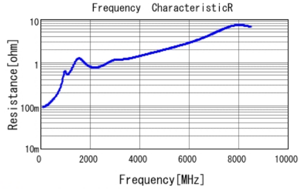
■ GRM1882C1H271JA01 R DCOV, 20degC
