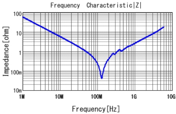
■ GRM1882C1H272JA01 |Z| DCOV, 20degC
