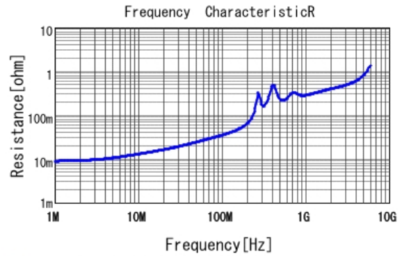
■ GRM1882C1H272JA01 R DCOV, 20degC
