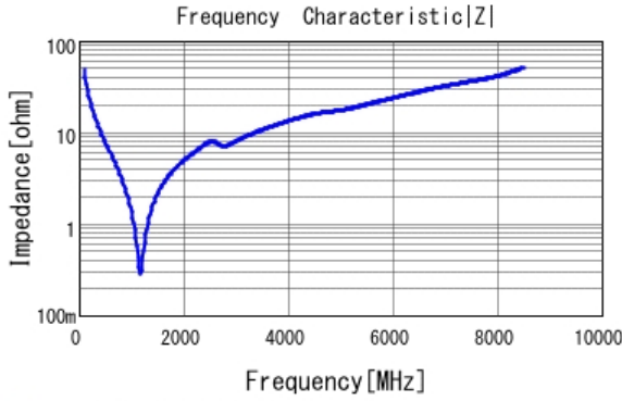
■ GRM1882C1H330JA01 |Z| DCOV, 20degC
