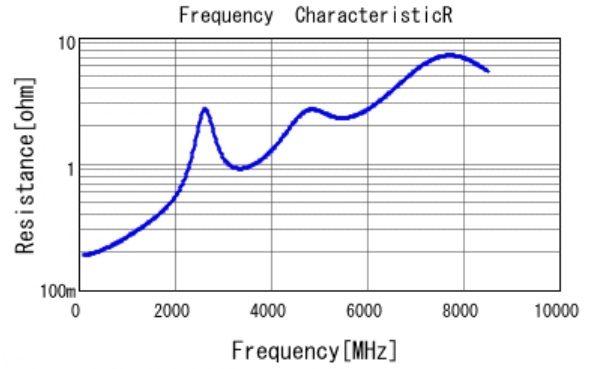
■ GRM1882C1H330JA01 R DCOV, 20degC
