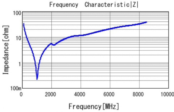
■ GRM1882C1H470JA01 |Z| DCOV, 20degC
