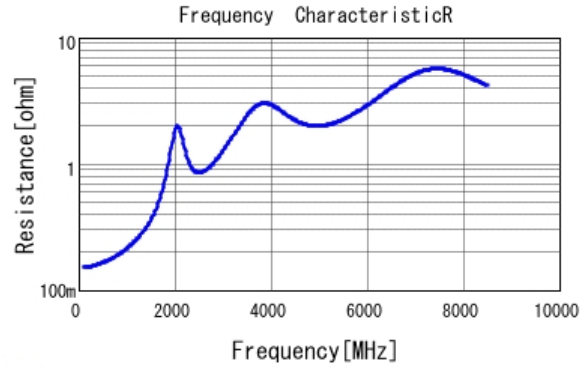
■ GRM1882C1H470JA01 R DCOV, 20degC
