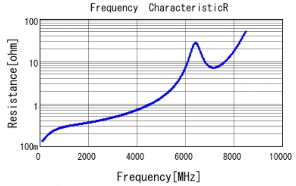
■ GRM1882C1H5R0CA01 R DCOV, 20degC
