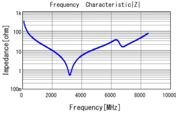
■ GRM1882C1H5R0CA01 |Z| DCOV, 20degC
