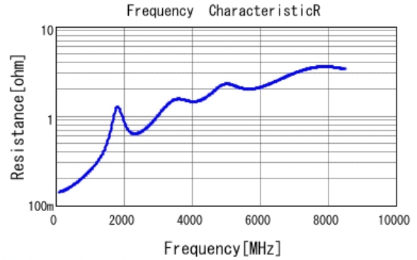
■ GRM1882C1H680JA01 R DCOV, 20degC
