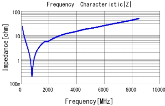
■ GRM1882C1H680JA01 |Z| DCOV, 20degC
