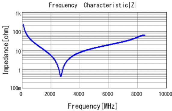
■ GRM1882C1H7R0DA01 |Z| DCOV, 20degC
