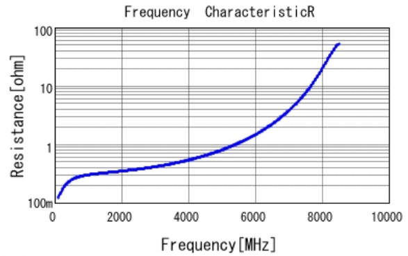
■ GRM1882C1H7R0DA01 R DCOV, 20degC
