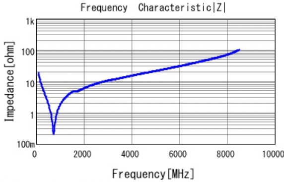
■ GRM1882C1H820JA01 |Z| DCOV, 20degC
