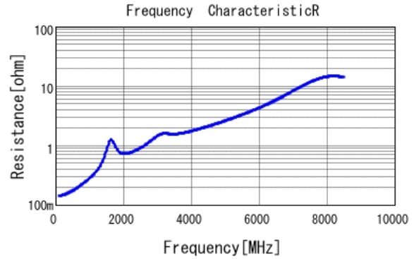
■ GRM1882C1H820JA01 R DCOV, 20degC
