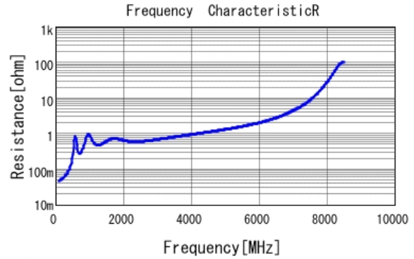
■ GRM1882C2A561JA01 R DCOV, 20degC
