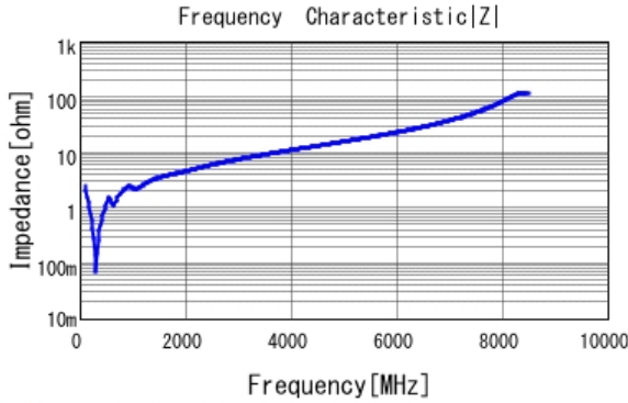
■ GRM1882C2A561JA01 |Z| DCOV, 20degC
