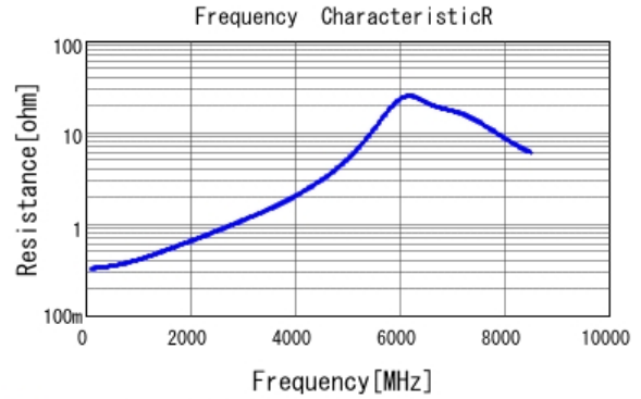
■ GRM1885C1H100JA01 R DCOV, 25degC
