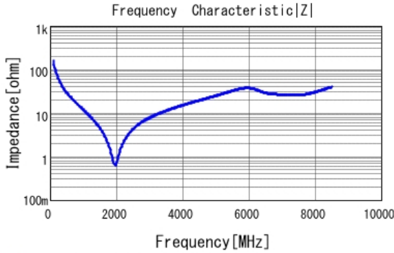
■ GRM1885C1H100JA01 |Z| DCOV, 25degC
