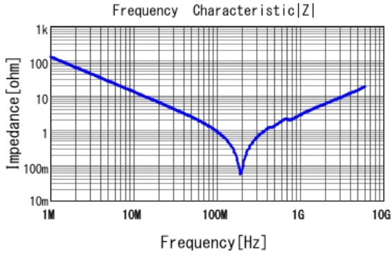
■ GRM1885C1H122JA01 |Z| DCOV, 25degC
