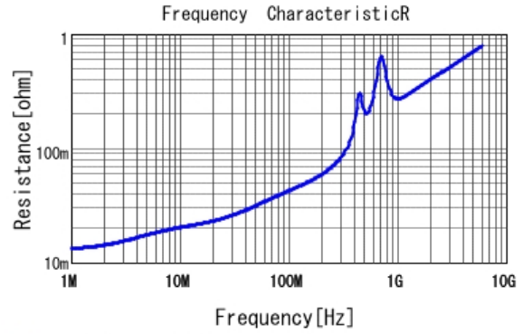
■ GRM1885C1H122JA01 R DCOV, 25degC
