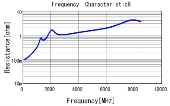
■ GRM1885C1H151JA01 R DCOV, 25degC
