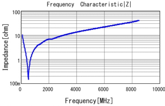
■ GRM1885C1H151JA01 |Z| DCOV, 25degC
