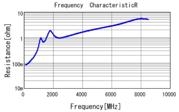
■ GRM1885C1H181JA01 R DCOV, 25degC
