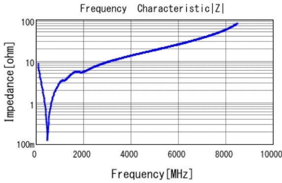
■ GRM1885C1H181JA01 |Z| DCOV, 25degC
