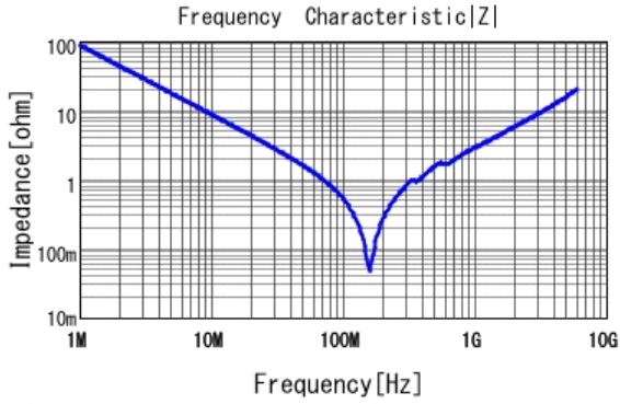
■ GRM1885C1H182JA01 |Z| DCOV, 25degC
