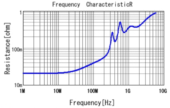
■ GRM1885C1H182JA01 R DCOV, 25degC
