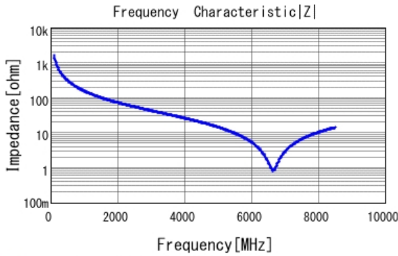
■ GRM1885C1H1R0WA01 |Z| DCOV, 25degC
