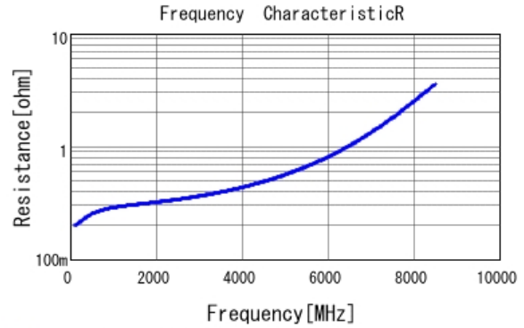
■ GRM1885C1H1R1BA01 R DCOV, 25degC
