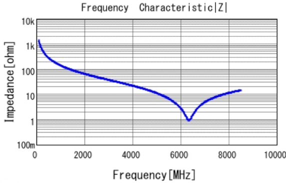
■ GRM1885C1H1R1BA01 |Z| DCOV, 25degC
