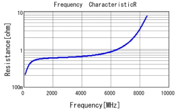
■ GRM1885C1H1R5BA01 R DCOV, 25degC
