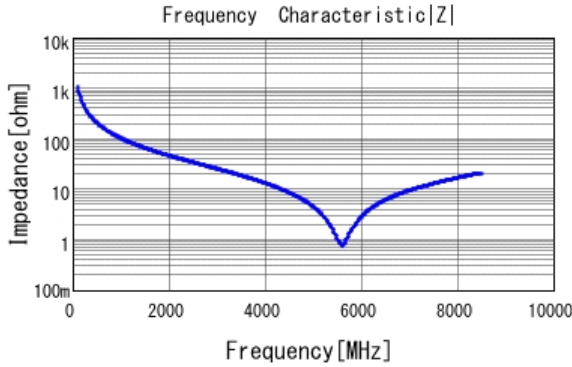
■ GRM1885C1H1R5BA01 |Z| DCOV, 25degC
