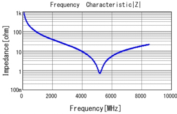
■ GRM1885C1H1R8BA01 |Z| DCOV, 25degC
