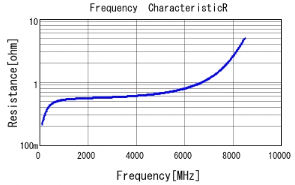
■ GRM1885C1H1R8BA01 R DCOV, 25degC
