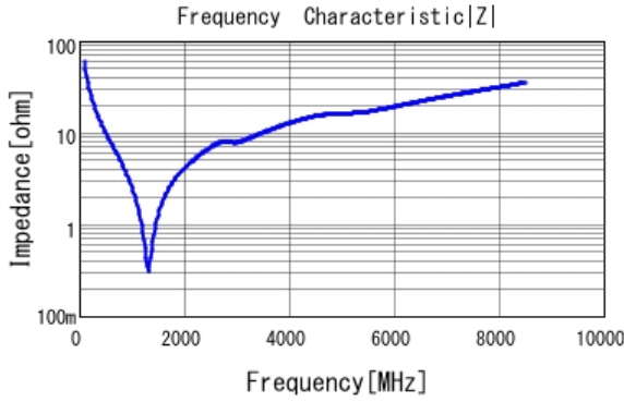
■ GRM1885C1H270JA01 |Z| DCOV, 25degC
