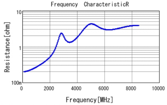
■ GRM1885C1H270JA01 R DCOV, 25degC
