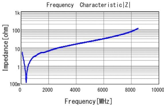
■ GRM1885C1H271JA01 |Z| DCOV, 25degC
