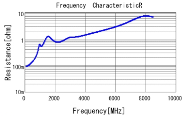
■ GRM1885C1H271JA01 R DCOV, 25degC
