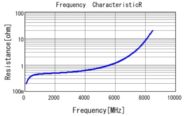
■ GRM1885C1H2R0BA01 R DCOV, 25degC
