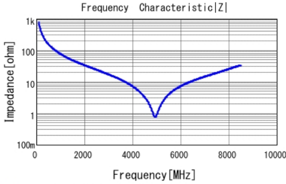
■ GRM1885C1H2R0BA01 |Z| DCOV, 25degC
