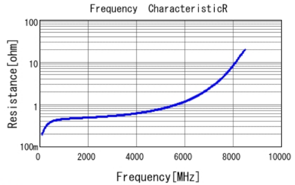
■ GRM1885C1H2R2BA01 R DCOV, 25degC
