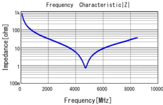
■ GRM1885C1H2R2BA01 |Z| DCOV, 25degC
