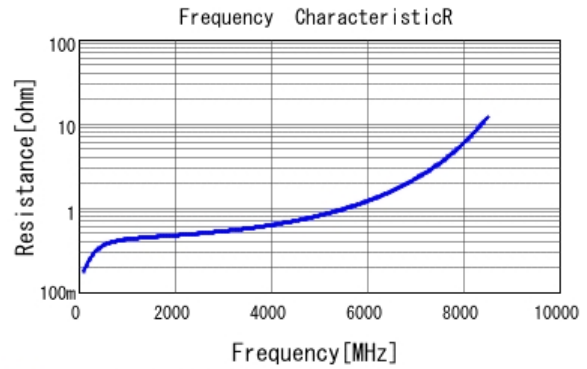
■ GRM1885C1H2R4BA01 R DCOV, 25degC
