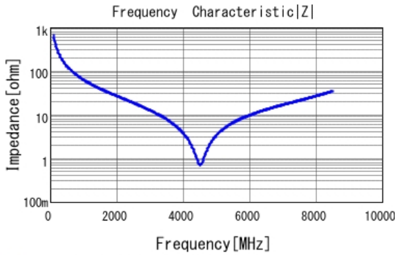
■ GRM1885C1H2R4BA01 |Z| DCOV, 25degC
