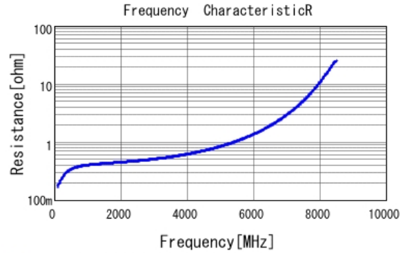
■ GRM1885C1H2R7BA01 R DCOV, 25degC
