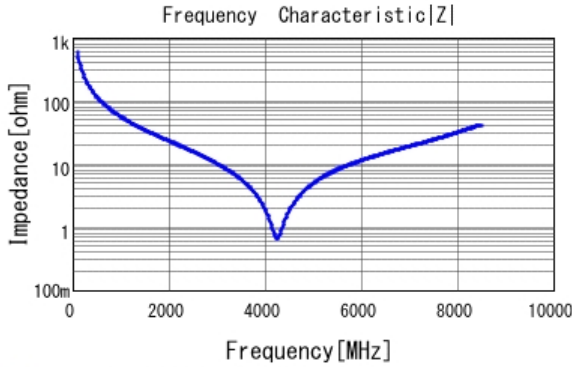
■ GRM1885C1H2R7BA01 |Z| DCOV, 25degC
