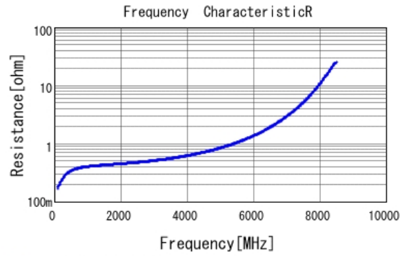
■ GRM1885C1H2R7CA01 R DCOV, 25degC
