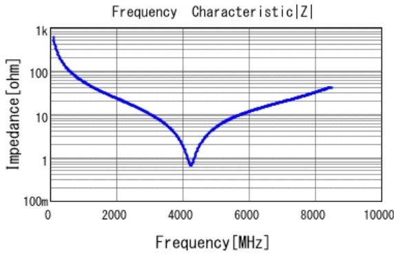
■ GRM1885C1H2R7CA01 |Z| DCOV, 25degC
