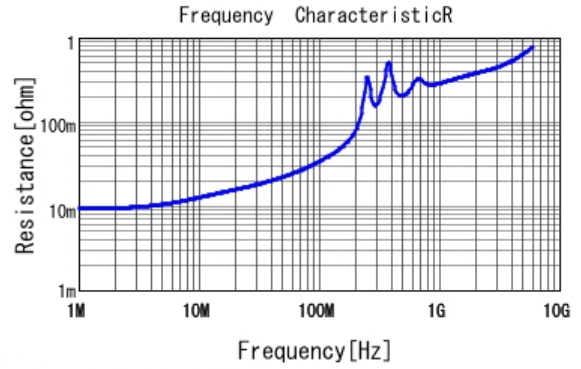
■ GRM1885C1H302JA01 R DCOV, 25degC
