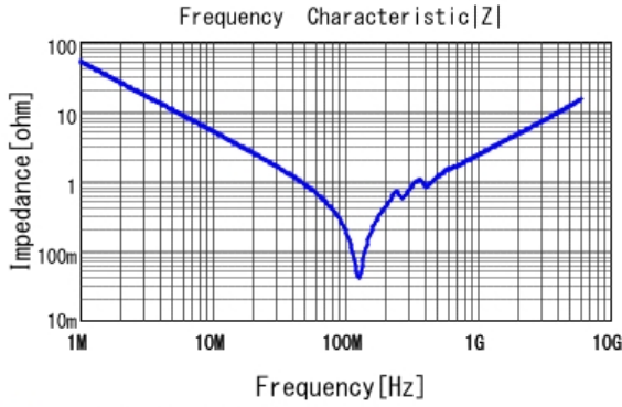
■ GRM1885C1H302JA01 |Z| DCOV, 25degC
