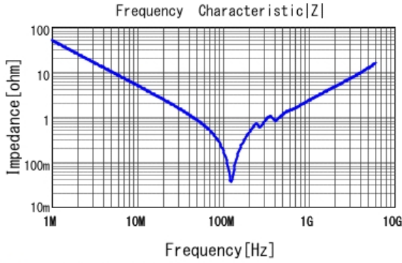
■ GRM1885C1H332JA01 |Z| DCOV, 25degC
