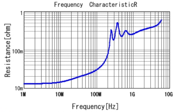
■ GRM1885C1H332JA01 R DCOV, 25degC
