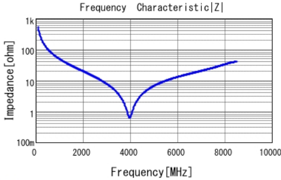
■ GRM1885C1H3R0CA01 |Z| DCOV, 25degC
