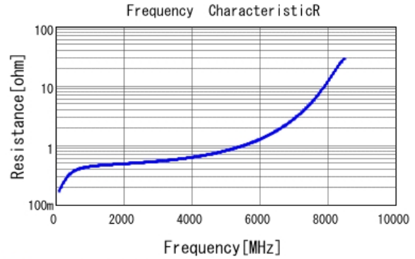
■ GRM1885C1H3R0CA01 R DCOV, 25degC
