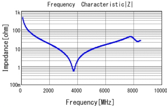
■ GRM1885C1H3R5BA01 |Z| DCOV, 25degC
