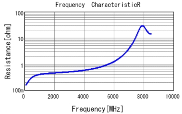
■ GRM1885C1H3R5BA01 R DCOV, 25degC
