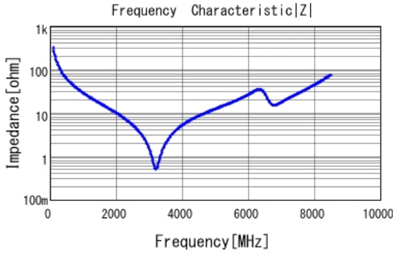
■ GRM1885C1H5R0CA01 |Z| DCOV, 25degC
