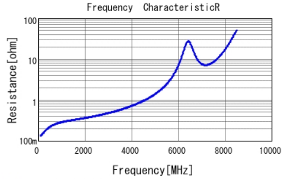
■ GRM1885C1H5R0CA01 R DCOV, 25degC
