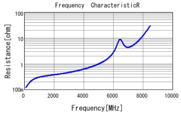
■ GRM1885C1H6R2DA01 R DCOV, 25degC
