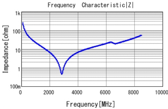
■ GRM1885C1H6R2DA01 |Z| DCOV, 25degC
