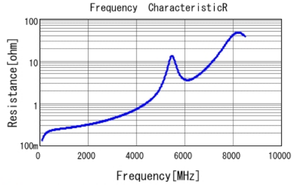
■ GRM1885C1H7R5CA01 R DCOV, 25degC
