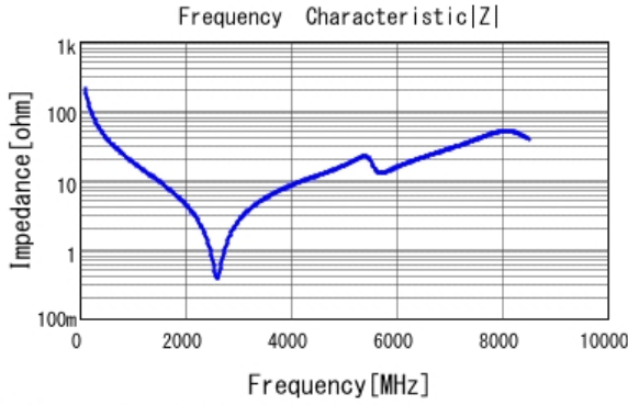
■ GRM1885C1H7R5CA01 |Z| DCOV, 25degC
