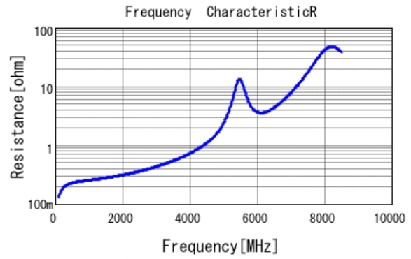
■ GRM1885C1H7R6BA01 R DCOV, 25degC
