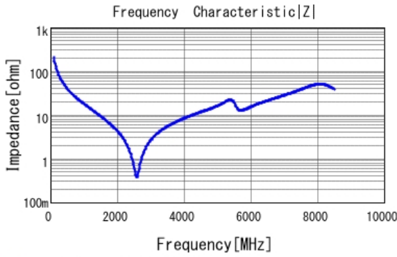
■ GRM1885C1H7R6BA01 |Z| DCOV, 25degC
