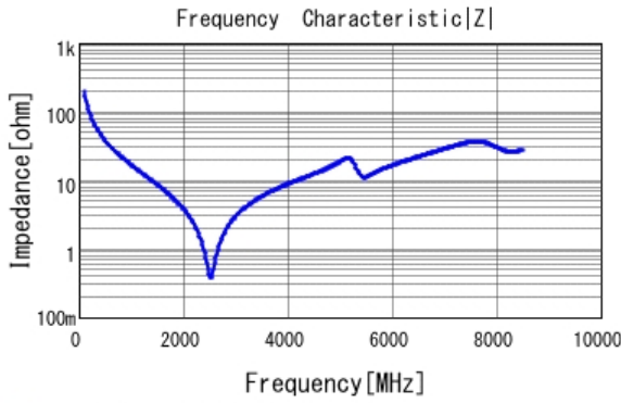
■ GRM1885C1H8R0CA01 |Z| DCOV, 25degC
