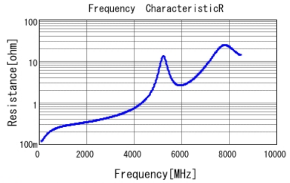
■ GRM1885C1H8R0CA01 R DCOV, 25degC
