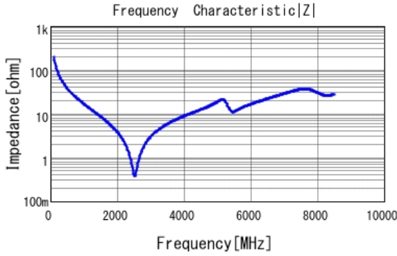
■ GRM1885C1H8R0DA01 |Z| DCOV, 25degC
