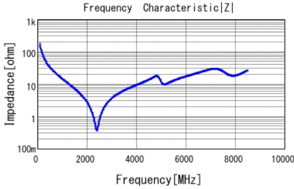
■ GRM1885C1H9R0BA01 |Z| DCOV, 25degC
