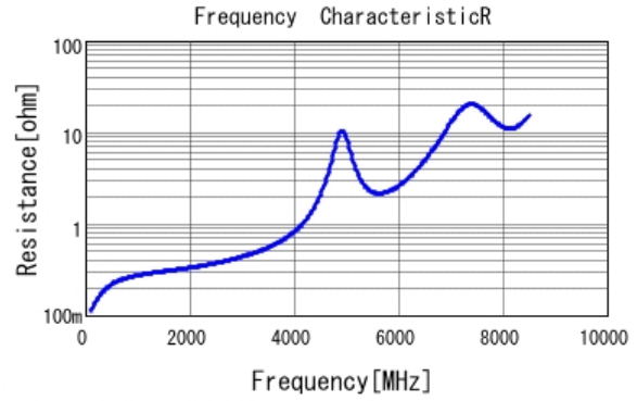
■ GRM1885C1H9R0BA01 R DCOV, 25degC
