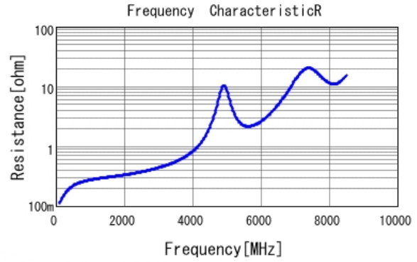
■ GRM1885C1H9R0CA01 R DCOV, 25degC
