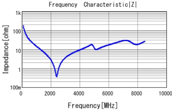
■ GRM1885C1H9R0DA01 |Z| DCOV, 25degC
