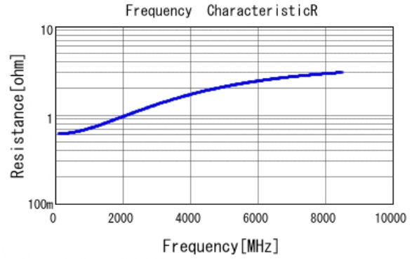
■ GRM1885C1HR50BA01 R DCOV, 25degC
