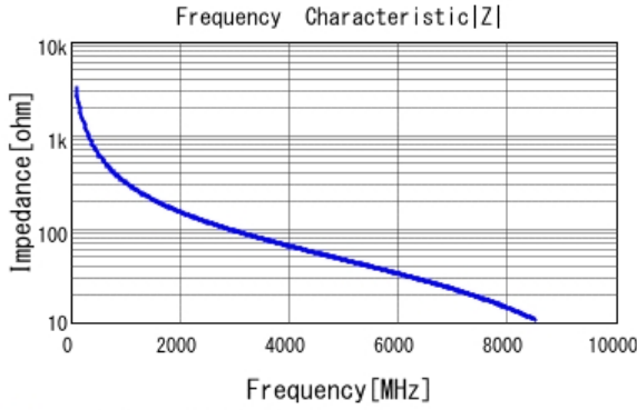
■ GRM1885C1HR50BA01 |Z| DCOV, 25degC
