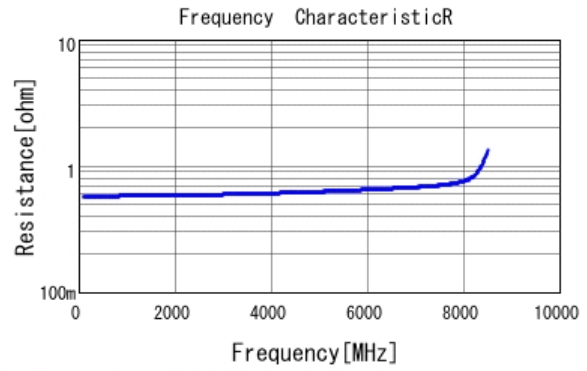
■ GRM1885C1HR60WA01 R DCOV, 25degC
