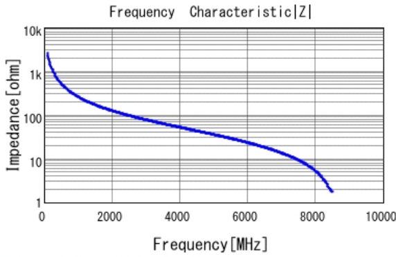
■ GRM1885C1HR60WA01 |Z| DCOV, 25degC
