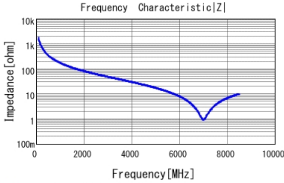
■ GRM1885C1HR90WA01 |Z| DCOV, 25degC
