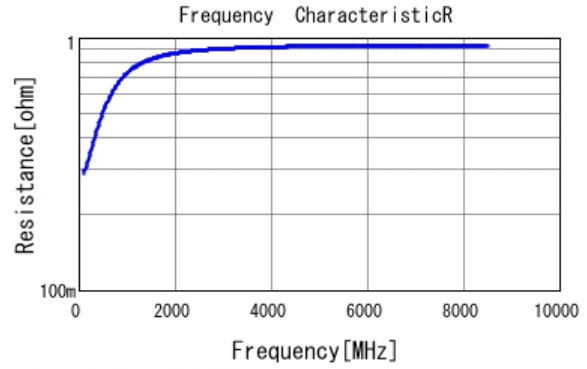
■ GRM1885C1HR90WA01 R DCOV, 25degC
