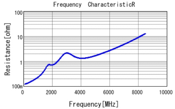
■ GRM1885C2A101JA01 R DCOV, 25degC
