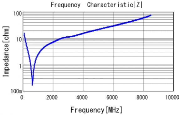
■ GRM1885C2A101JA01 |Z| DCOV, 25degC
