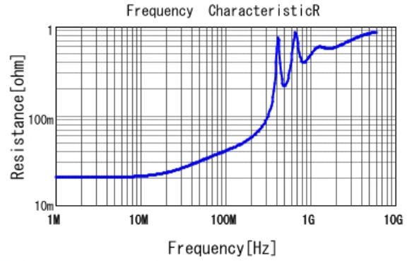
■ GRM1885C2A102JA01 R DCOV, 25degC
