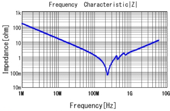
■ GRM1885C2A102JA01 |Z| DCOV, 25degC
