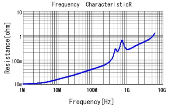
■ GRM1885C2A122JA01 R DCOV, 25degC
