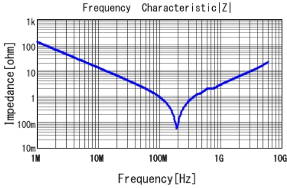
■ GRM1885C2A122JA01 |Z| DCOV, 25degC
