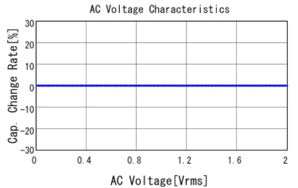
■ GRM1885C2A122JA01 C-AC Voltage capchange, DCOV, 25.0d
