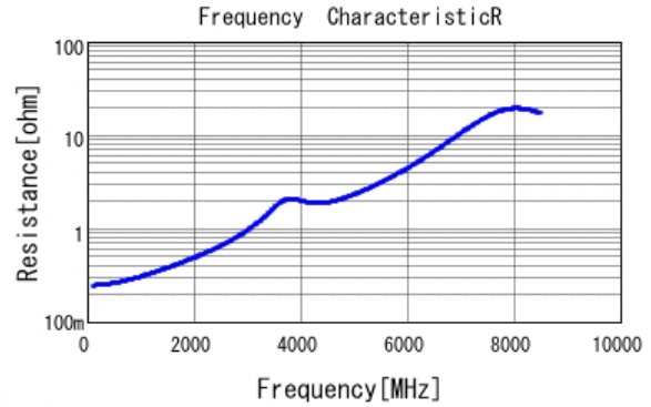
■ GRM1885C2A150JA01 R DCOV, 25degC
