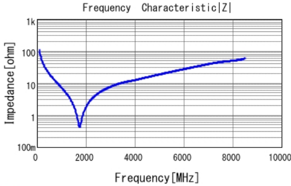
■ GRM1885C2A150JA01 |Z| DCOV, 25degC
