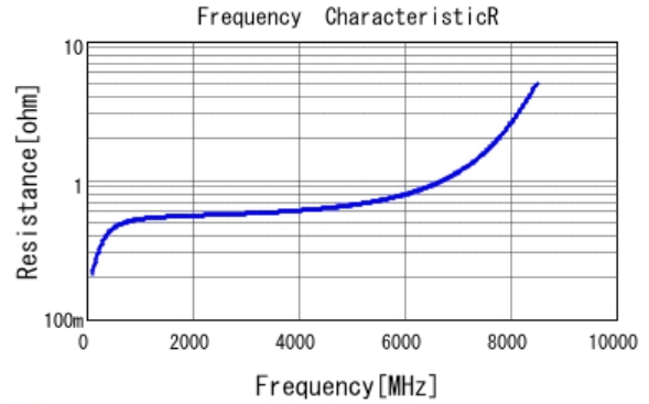
■ GRM1885C2A1R8BA01 R DCOV, 25degC
