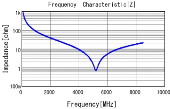
■ GRM1885C2A1R8BA01 |Z| DCOV, 25degC
