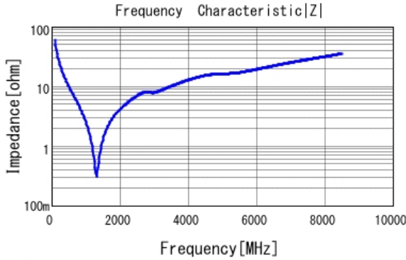
■ GRM1885C2A270JA01 |Z| DCOV, 25degC
